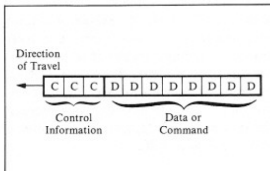
FIGURE 1-7. Structure of an HP-IL message
