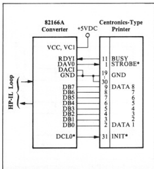
FIGURE 2-7. HP 82166A Converter to Centronics-type printer interface
